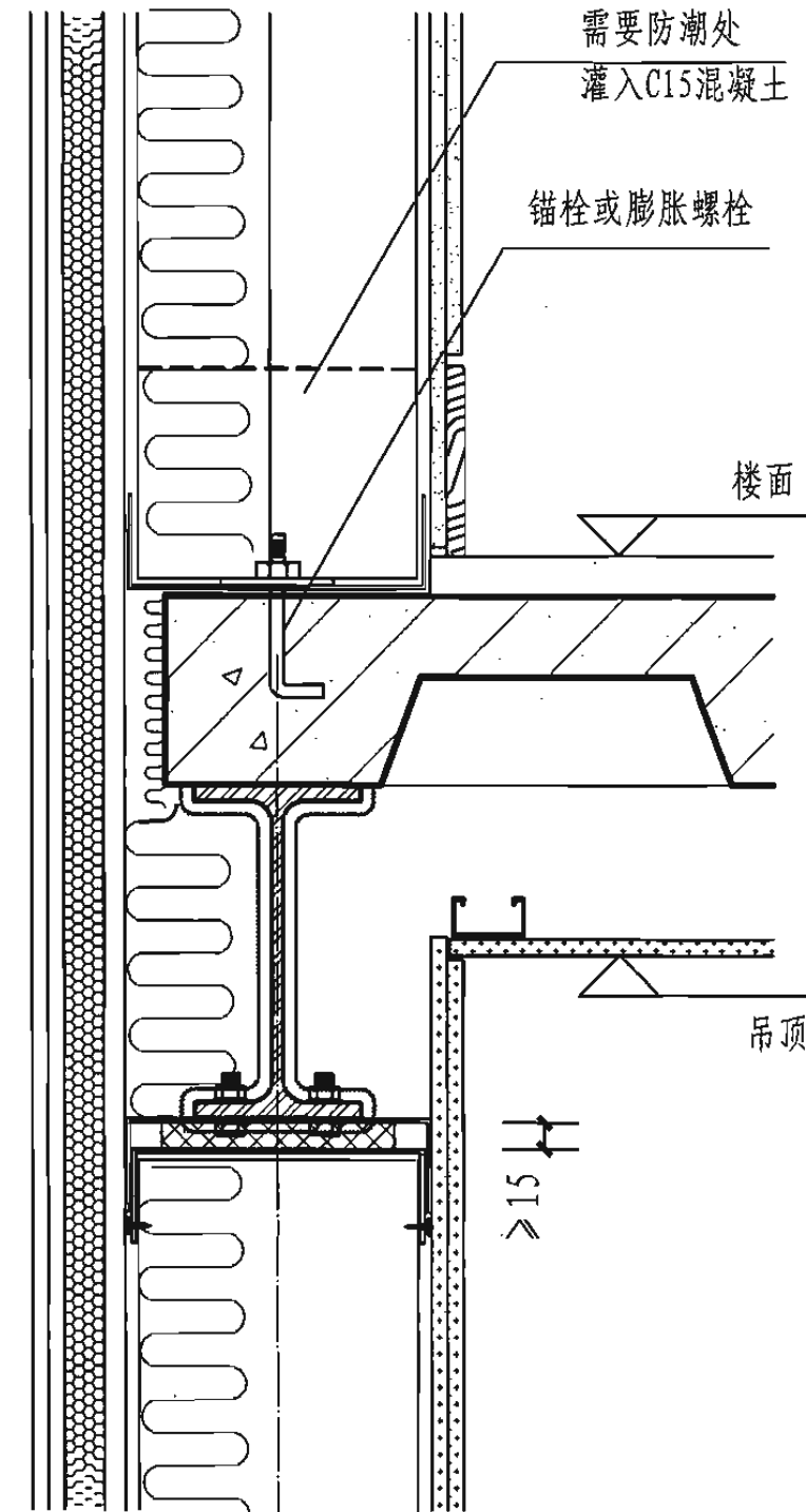
2-2
